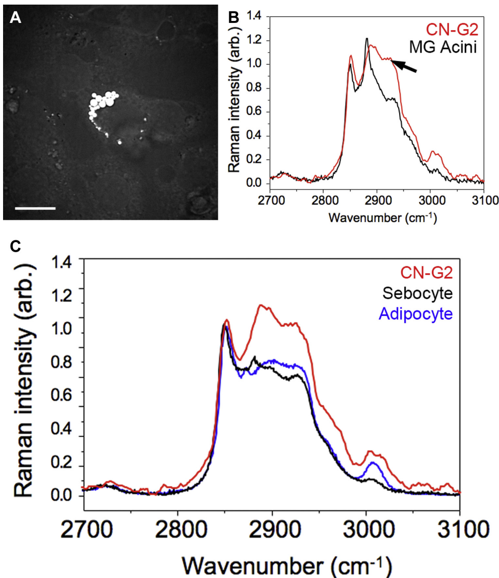
Figure 3. Coherent Anti-Stokes Raman (CARS) image focused on 2845 cm -1 (A) and Raman microspectroscopy (B and C) of CN-G2 lipid vacuoles. CN-G2 cells (B and C, Red line) show major peaks at 2846 cm -1 and 2886 cm -1 , similar to that of lipid within meibomian gland acini (B) indicating the abundance of wax and cholesterol esters, respectively. Lipid in CN-G2 cells was distinct from that of lipid within sebocytes and adipocytes (C, black and blue, respectively), which contain reduced cholesterol esters. Also note the presence of an elevated peak at 2940 cm -1 from the CH 3 stretch region representative of protein in CN-G2 cells (B, arrow) that is also present in acinar lipid at reduced levels that show maturational changes within the meibomian gland lipid.
