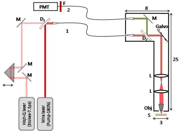
Fig. 1. Schematic diagram of the fiber-delivered probe for CARS tissue imaging: M- mirrors; D1- 1000 nm longpass dichroic mirror; D2- 760 nm longpass dichroic mirror, L-lens; Obj-objective; S-sample; F- 670 nm bandpass filter. Fiber 1 is used for delivery of the excitation pulses and fiber 2 is used for detecting the CARS radiation. The dimensions of the probe are indicated in cm.
