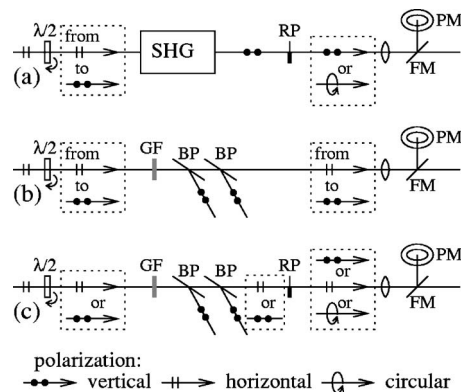
FIG. 10. Transformation of the pump beam in view of the intensity scaling for the two polarizations used. Pumping with (a) 405\text{ nm} , linear or circular polarizations; (b) 810\text{ nm} , linear polarization; (c) 810\text{ nm} , linear or circular polarizations. \lambda/2 : half-wave plate, SHG: second-harmonic generation, RP: tunable retardation plate, BP: Brewster plate, GF: thin gray filter, FM: flipping mirror, and PM: power meter.
