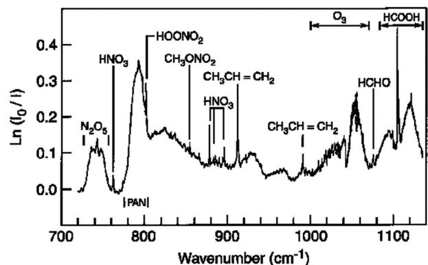
Figure 13. Typical infrared spectrum of irradiated VOC-NOx mixture in air.
