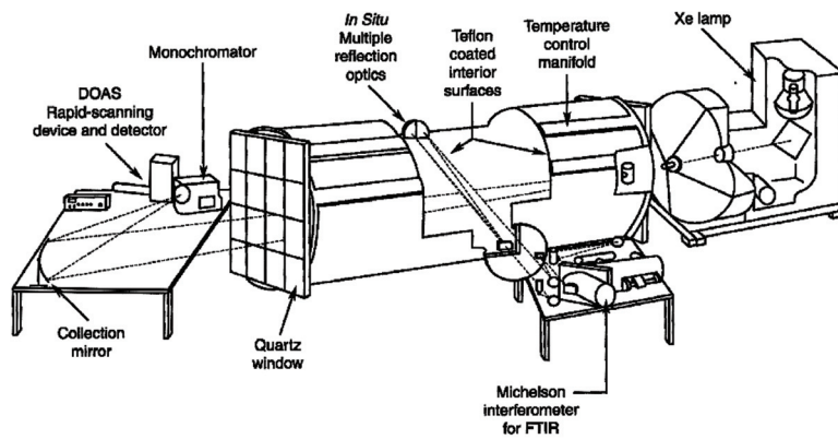
Figure 11. Schematic diagram of the SAPRC environmental chamber.
