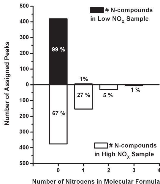
Figure 3. The distribution of NOC compounds in SOA generated from the low- and high- \text{NO}_x photooxidation of isoprene. Most particle-phase compounds do not contain nitrogen even when generated under high initial \text{NO}_x concentrations; however, a significant fraction of high- \text{NO}_x SOA molecules contain one (27%), two (5%), and three (1%) nitrogen atoms.
