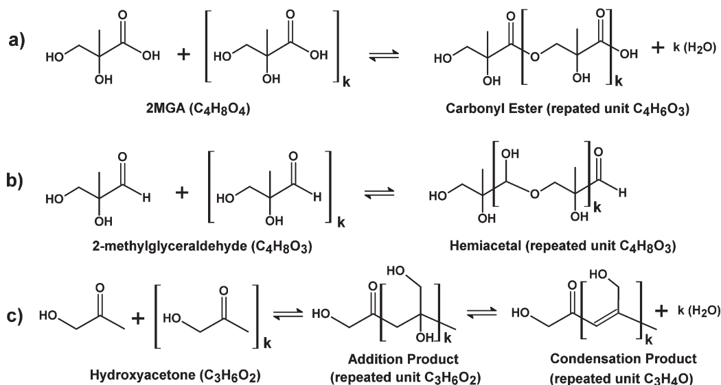
Figure 5. Illustrative examples of self-oligomerization reactions of (a) 2-methylglyceric acid (2MGA) producing carbonyl esters through condensation chemistry from repeated integration of C_4H_6O_3 units (b) 2-methylglyceraldehyde producing linear hemiacetals through addition chemistry from repeated integration of C_4H_8O_3 units and (c) hydroxyacetone producing an aldol through addition chemistry from repeated integration of C_3H_6O_2 units, followed by the formation of an aldol condensation product via loss of H_2O , which results in repeated C_3H_4O units.
