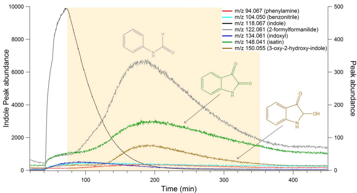
Figure S2.3: Time-dependent signals of ions that were produced and then removed
