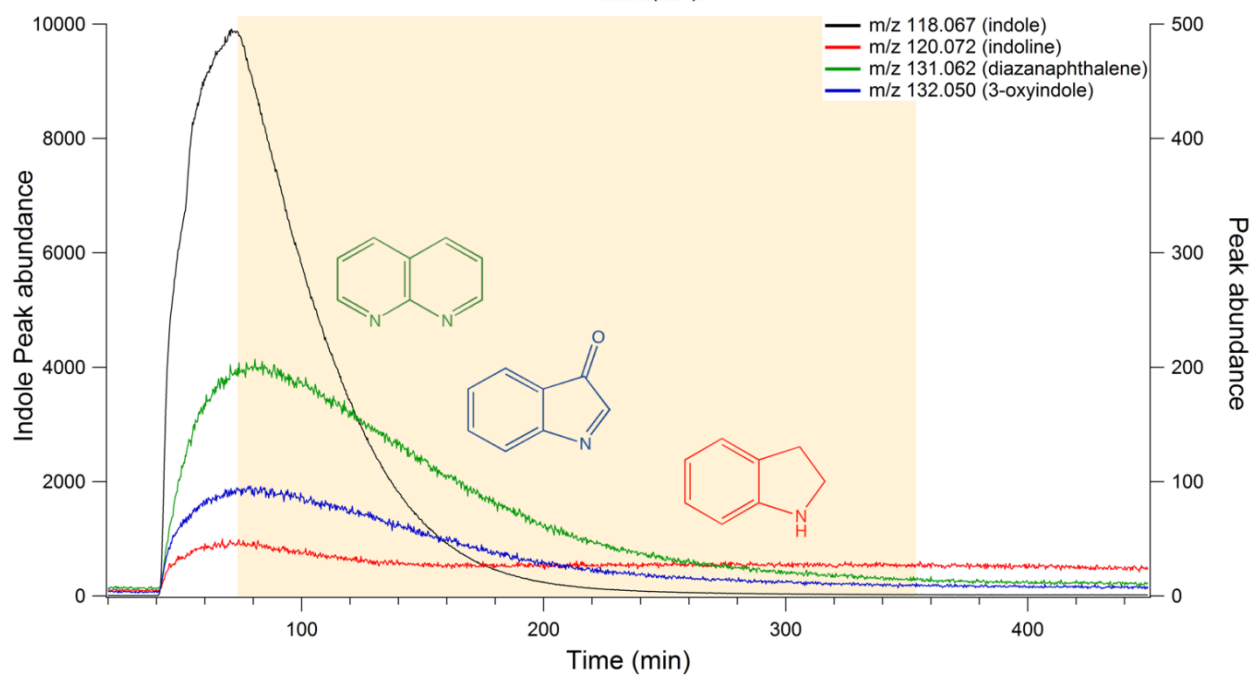
Figure S2.4: Time-dependent signals of ions that were removed during photooxidation
