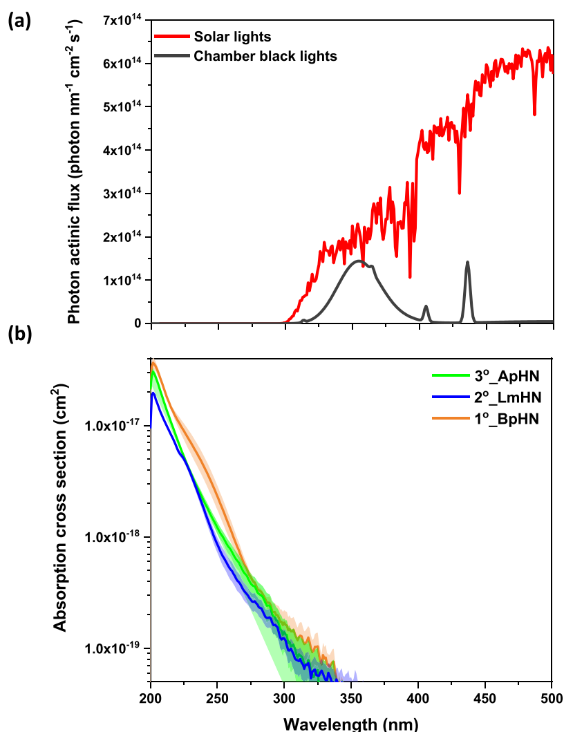
Figure 3. (a) Comparison between GTEC chamber black lights and solar spectral photon flux (extracted from TUV-radiation model, solar zenith angle of 28.14°, 12:00 solar time, August 1 at 33.75° latitude north (Atlanta), overhead O 3 column 300 Du, and albedo 0.1). (b) Absorption cross sections of 3°_ApHN, 2°_LmHN, and 1°_BpHN in ethyl ether. The uncertainties in the shaded areas were from the average of measured absorption cross sections in different solution concentrations.
