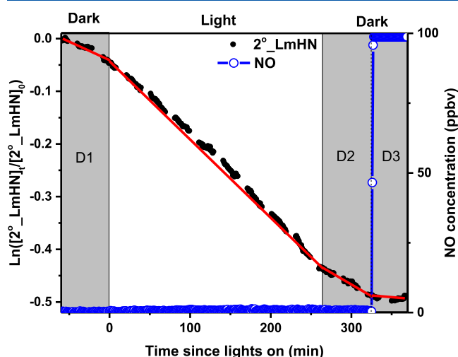
Figure 2. First-order kinetics analysis for photolysis of 2°_LmHN. The red line in each period corresponds to first-order kinetics fitting curve. D1 is the dark period before irradiation time (light on). D2 and D3 are dark periods after irradiation time. Detailed discussion for each period is provided in section 2.2.
