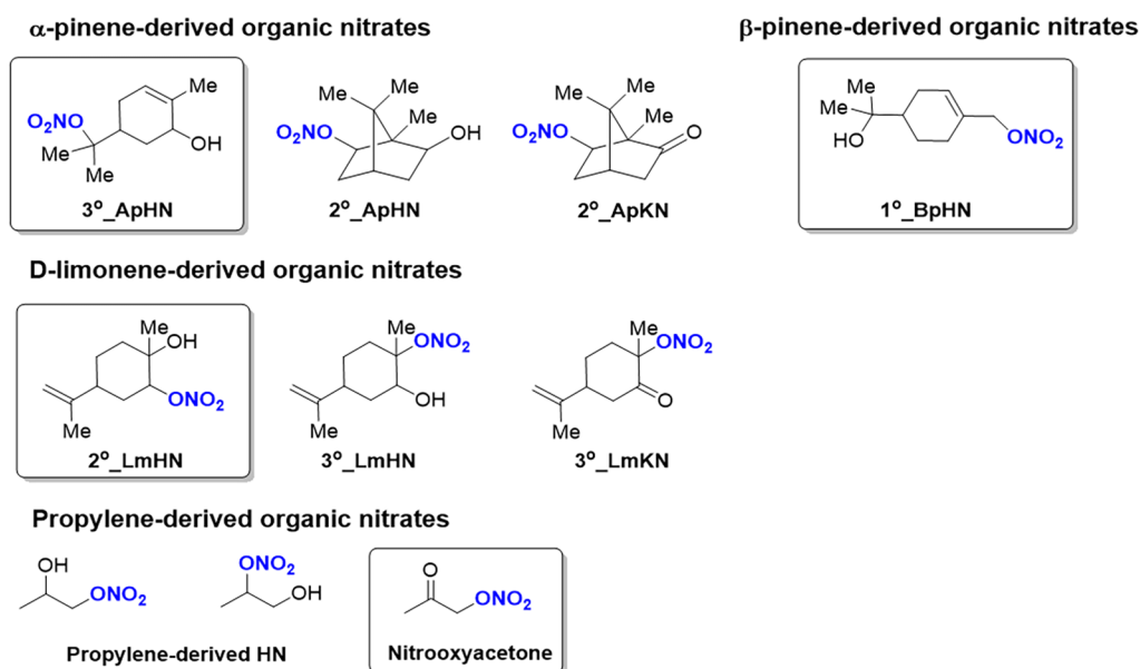
Figure 1. Molecular structures of ONs (HN: hydroxy nitrates and KN: keto-nitrates) synthesized in this work and their abbreviations. The numbers ( 1^\circ , 2^\circ , and 3^\circ ) in the abbreviations denote a primary, secondary, and tertiary nitrooxy group, respectively. The ONs in the boxes were introduced into the chamber to study the photolysis process.
