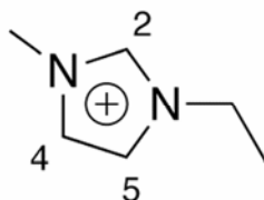
Figure 1.4. Example of imidazolium cation structure (i.e., [\text{C}_2\text{MIM}]^+ ) with carbons on the imidazolium ring labeled.
