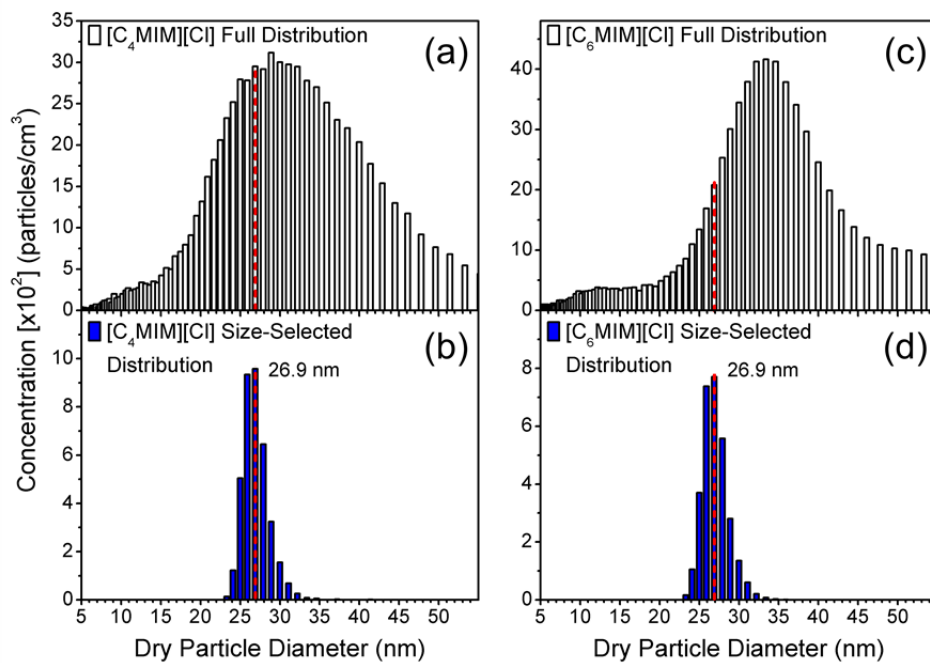
Figure 5.2. Full particle mobility size distributions of the dry [C 4 MIM][Cl] (a) and [C 6 MIM][Cl] (c) particles measured by the first nano-differential mobility analyzer (nano-DMA); the mobility size distributions after size selection for 26.9 \pm 0.01 nm [C 4 MIM][Cl] (b) and [C 6 MIM][Cl] (d) particles measured by the second nano-DMA. The red, dotted lines indicate where the dry size-selected particle distributions were located in the full particle distributions.
