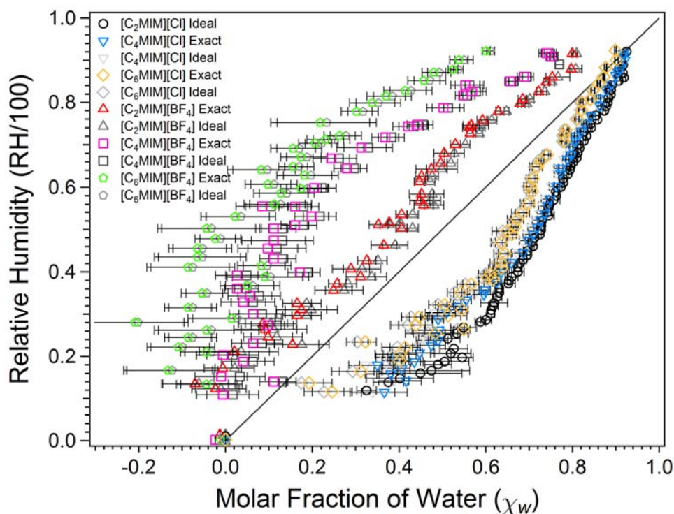
Figure 5.10. Water activity (RH/100) as a function of the molar fraction of water ( \chi_w ), calculated from the growth factor values using eq 4.1 (actual densities) and eq 4.2 (ideal solution approximation). The \chi_w data from our previous study, 1 [C 2 MIM][Cl] (black circles) and [C 2 MIM][BF 4 ] (red triangles), are included for comparison. Raoult's law for an ideal solution is represented by the dark grey, solid line.
