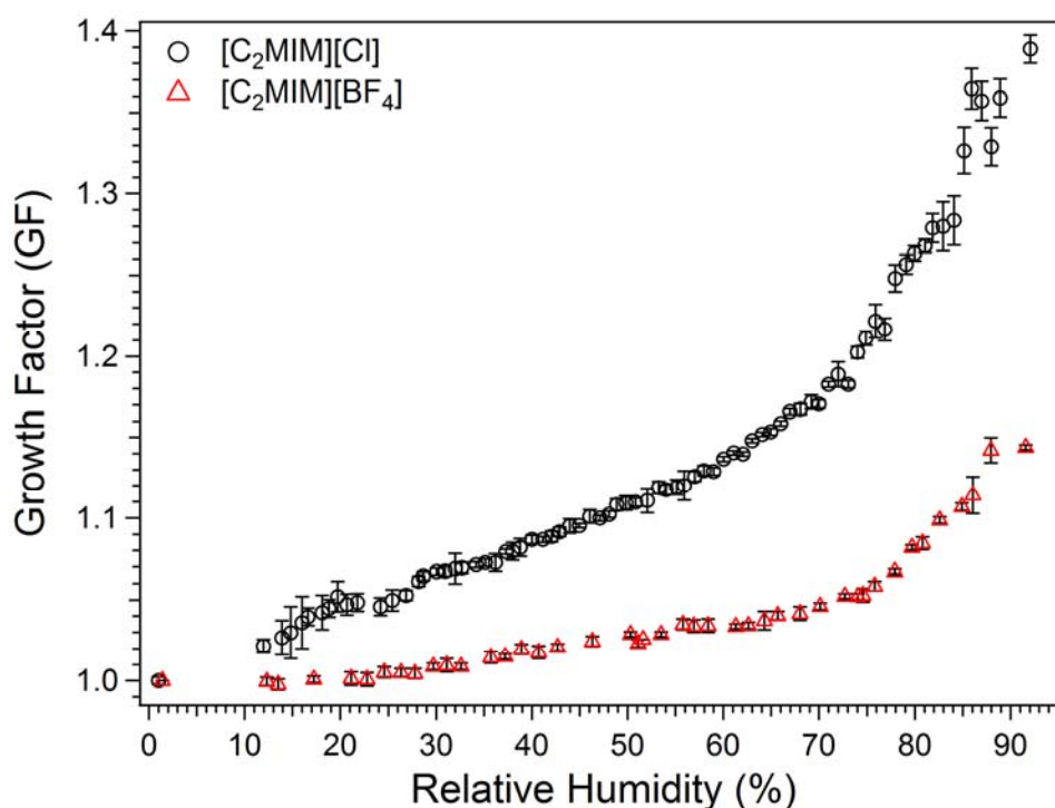
Figure 4.1. Hygroscopic growth curve of mobility-equivalent diameter selected 26.9 \pm 0.1 nm particles of [C 2 MIM][Cl] (circles) and [C 2 MIM][BF 4 ] (triangles). Both ionic liquids undergo a gradual increase in growth factor (GF) as the relative humidity is increased. [C 2 MIM][Cl] has a larger GF compared to [C 2 MIM][BF 4 ] and thus takes up more water.
