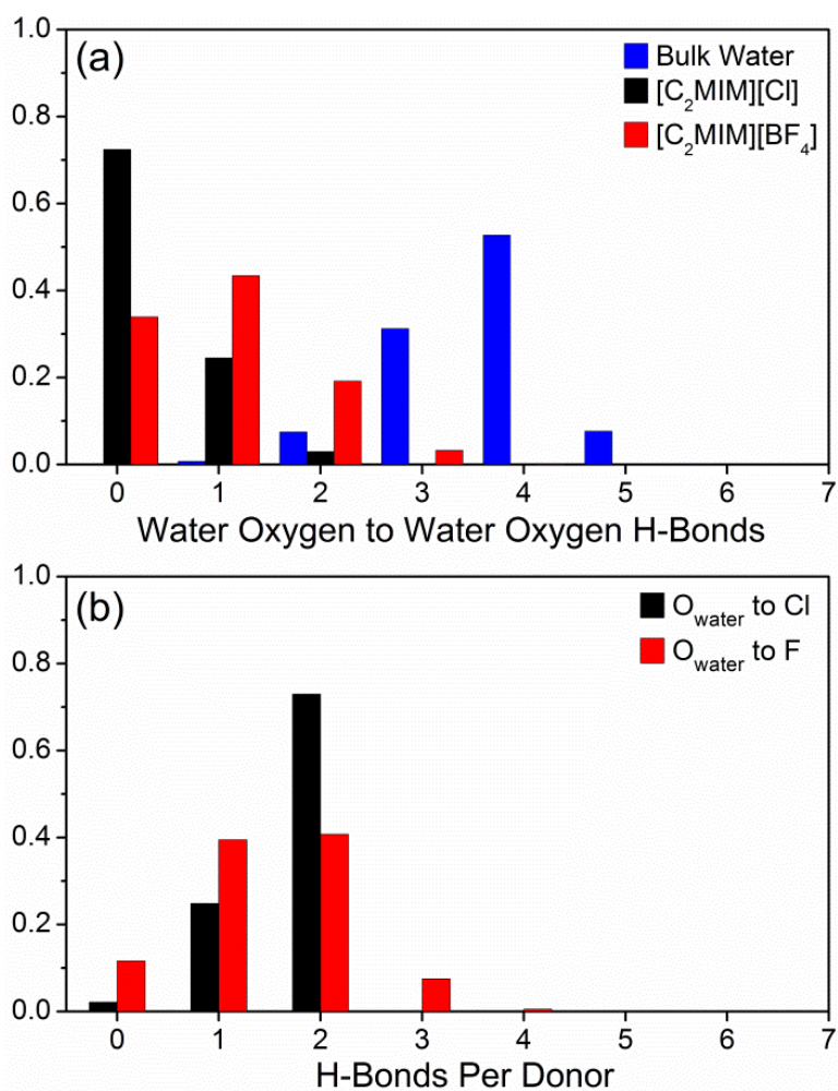
Figure 4.5. Hydrogen bond (H-bond) distribution histograms from MD simulation trajectories of (a) water oxygen ( \text{O}_{\text{water}} ) to \text{O}_{\text{water}} H-bonds in 1:1 mixtures of water with either bulk water, [\text{C}_2\text{MIM}][\text{Cl}] , or [\text{C}_2\text{MIM}][\text{BF}_4] and (b) \text{O}_{\text{water}} donor H-bonds to either chloride or fluorine anions.
