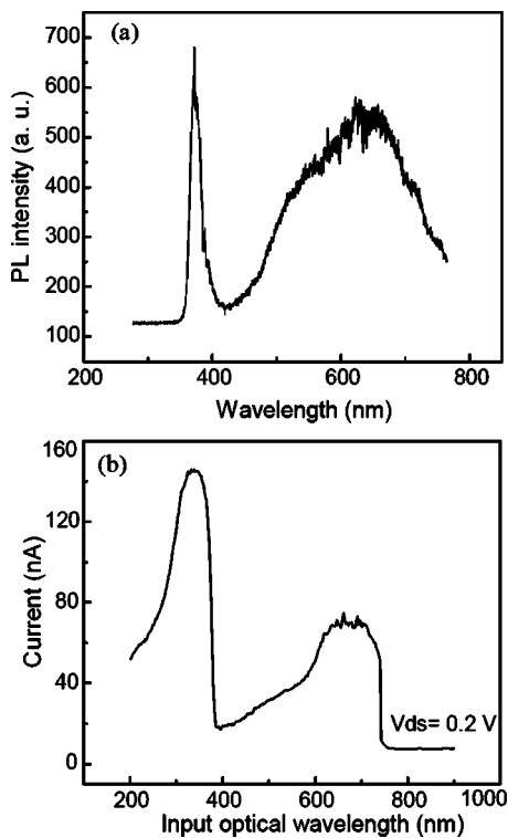
FIG. 2. (a) The PL of a ZnO NW excited with 351 nm UV laser. (b) The photoconductivity of a ZnO NW obtained at 0.2 V drain-source bias ( V_{ds} ).
